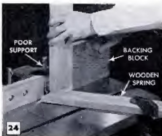
When the molding cut must run across the grain and on the face of the stock, use the setup pictured above. The setup shown at the left is permissible only on stock wider than 6 in.
